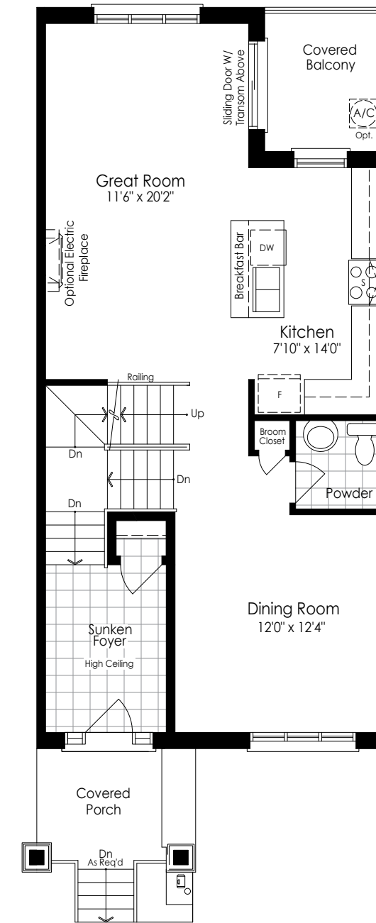
MAIN FLOOR Elevation A & B
